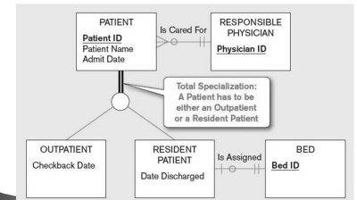
Figure 3-6 Examples of completeness constraints a) Total specialization rule
