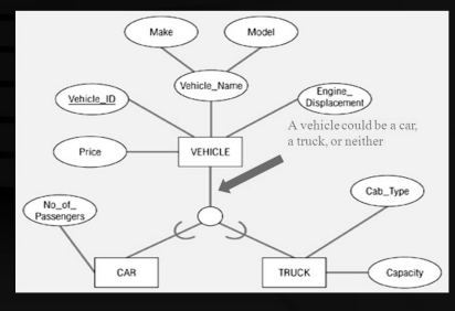
Figure 4-6b: Completeness Constraints - Partial Specialization Rule
