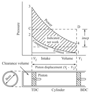
Fig. 16.1 p-V diagram for an ideal four-stroke cycle engine
